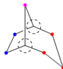
bicyclo[3.2.1]octane
