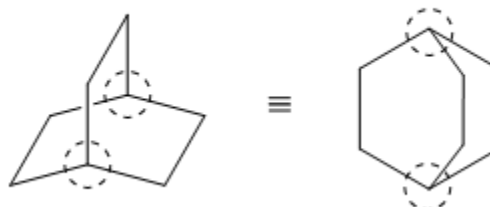
Bridged Bicyclic
