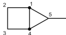
5-methylbicyclo[2.1.0]pentane
