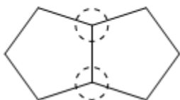
Normal Bicyclic
